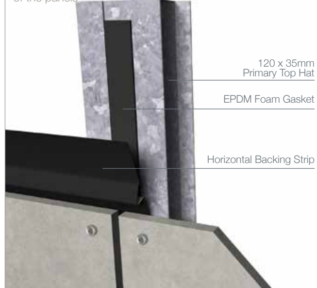
Figure 8 Inserting Horizontal Backing Strip along the top edge of the panels
