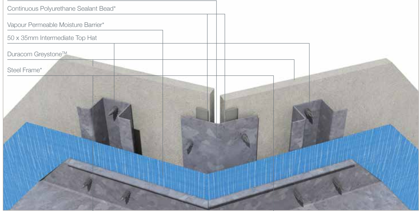
Figure 19 Angled Internal Corner Support Angle 60 x 60 x 1mm*
