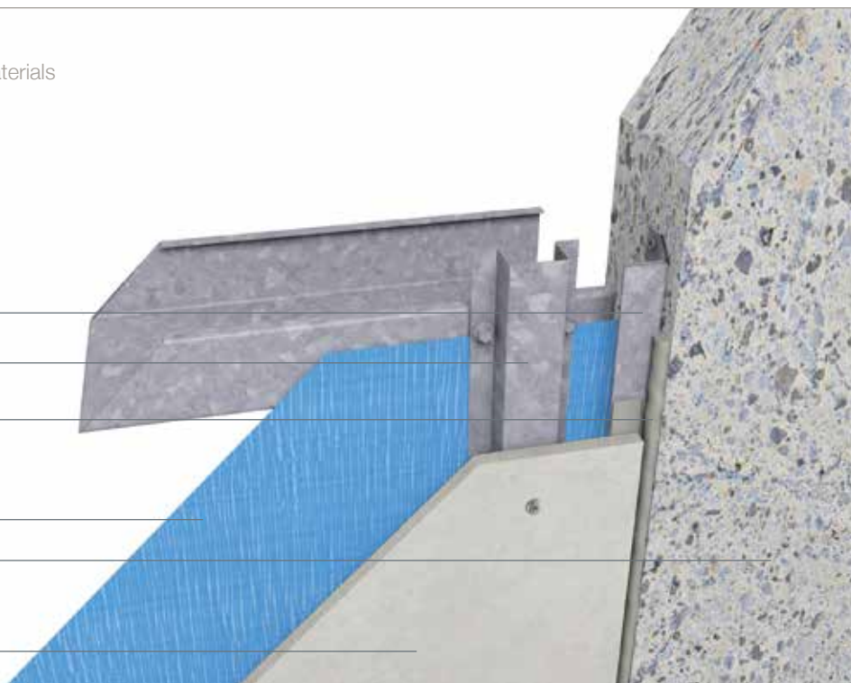
Figure 24 Vertical Control Joint
