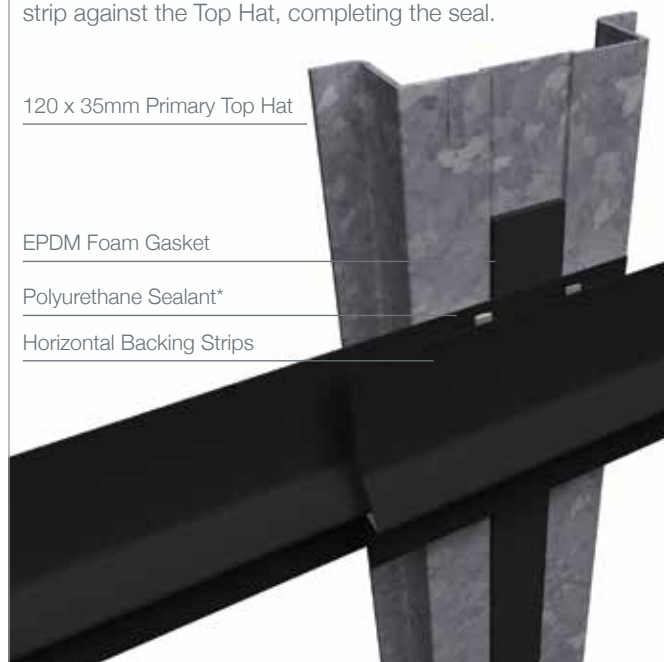
Figure 11 Installing Next Panel
