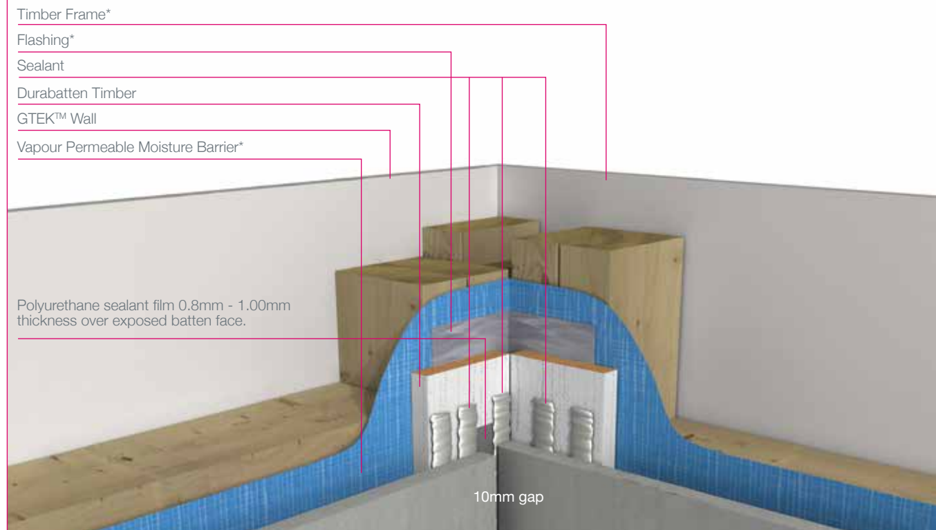
Figure 17 Internal Corner
