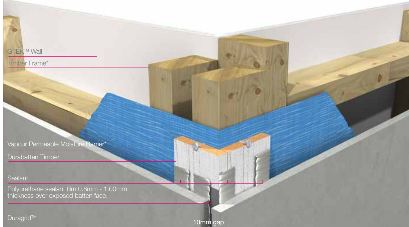
Figure 18 External Corner
